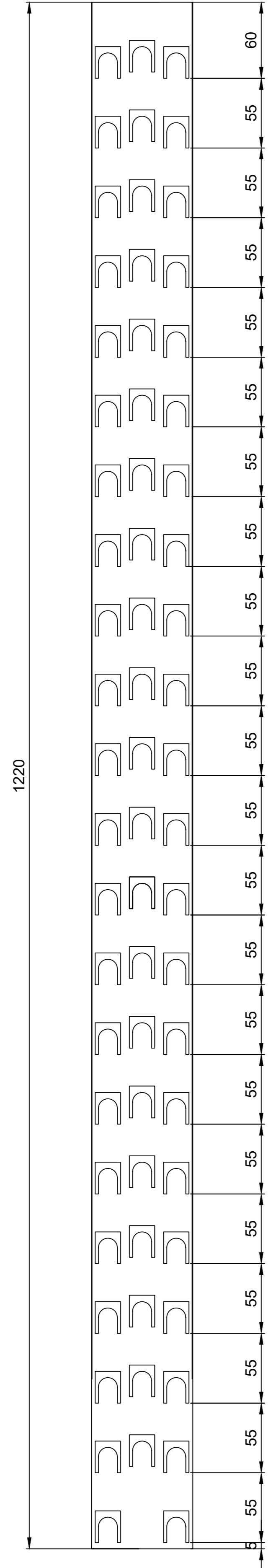
22 Lamellen
